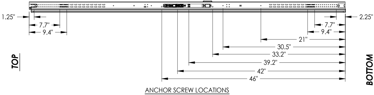
ANCHOR SCREW LOCATIONS
